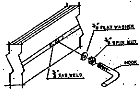
HOOK ASSEMBLY-TYP.
